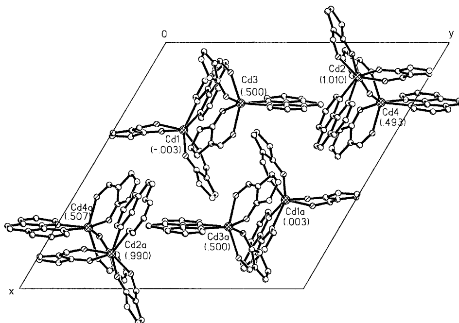
Fig. 5 Packing of [\text{Cd}(\text{Q}_\text{C})_2(\text{phen})] (4) molecules in the unit cell. The numbers in brackets indicate z coordinates of Cd atoms. All methyl, phenyl and cyclohexyl substituents as well as H atoms are omitted for clarity.
