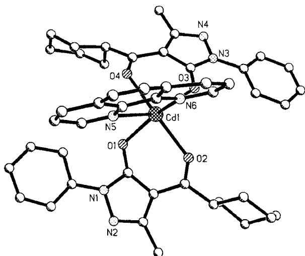
Fig. 4 Molecular structure of [\text{Cd}(\text{Q}_\text{C})_2(\text{phen})] (4) exemplified by the complex with Cd(1). H atoms are omitted for clarity.
